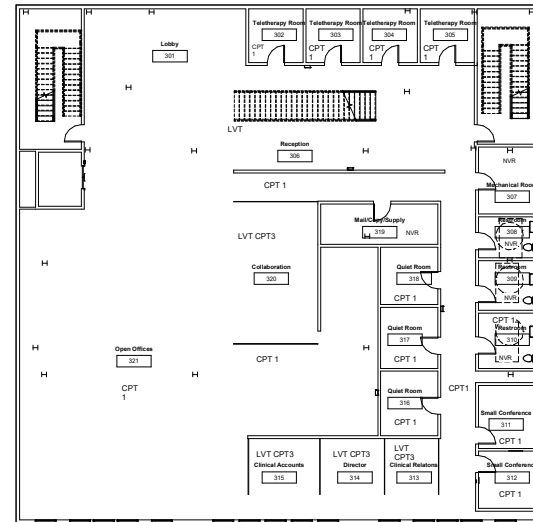
Finish plan third floor 1/8" = 1'-0"
