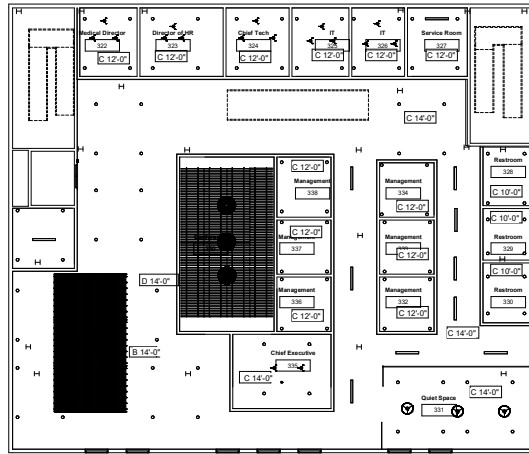
Level 2 1/8" = 1'-0"
