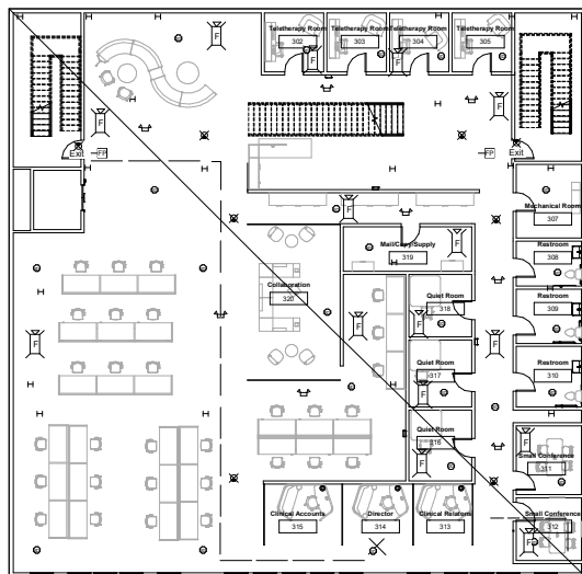
① Third Floor Life Safety 1/8" = 1'-0"
