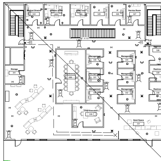
② Fourth Floor Life Safety 1/8" = 1'-0"
